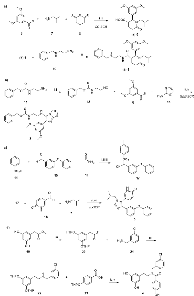
Scheme 1. Synthetic pathways of compounds 1-4. Reagents and conditions: a) Compound ( \pm )- 1 : i) 6 , 7 , HCOOH, ACN, mw 120°C, 50 W, 30 min; ii) 8 , p-xylene, reflux, 10 h,
