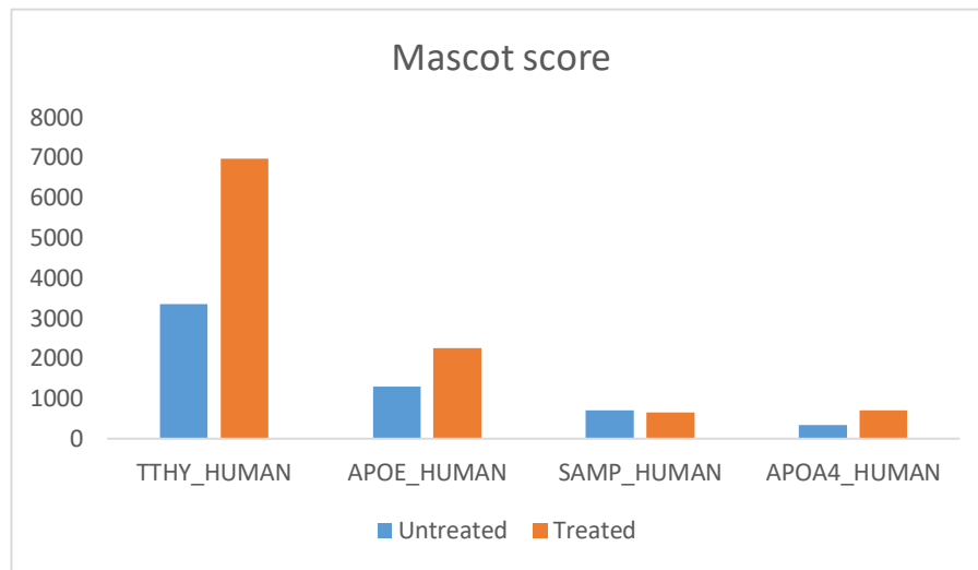
Supplementary Table S1: Effect of acetonitrile/TFA pre-treatment on amyloid protein score on paired FFPE tissues.
