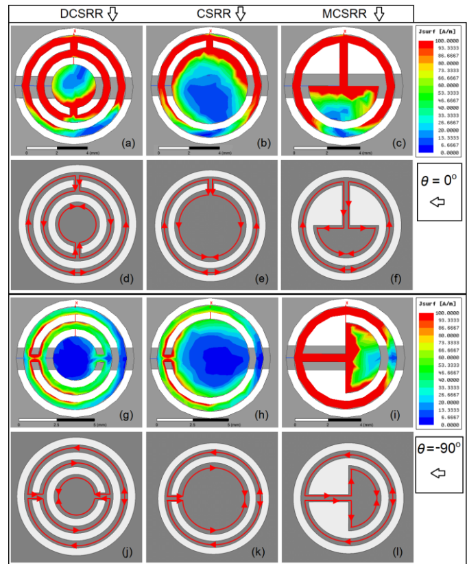
Figure 4. Magnitude plots of (a) DCSRR, (b) CSRR, and (c) MCSRR; vector plots of (d) DCSRR, (e) CSRR, and (f) MCSRR at \theta = 0^\circ ; magnitude plots of (g) DCSRR, (h) CSRR, and (i) MCSRR; vector plots of (j) DCSRR, (k) CSRR, and (l) MCSRR at \theta = -90^\circ (fixed dimensions are c = 3.5 mm, g = s = t = 0.5 mm).
