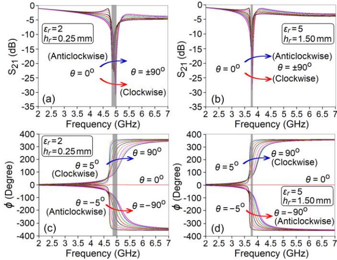
29 Figure 8. Frequency response of the magnitude of S_{21} for (a) rotor1 and (b) 30 rotor2; relative phase for (c) rotor1 and (d) rotor2 with respect to \theta .
