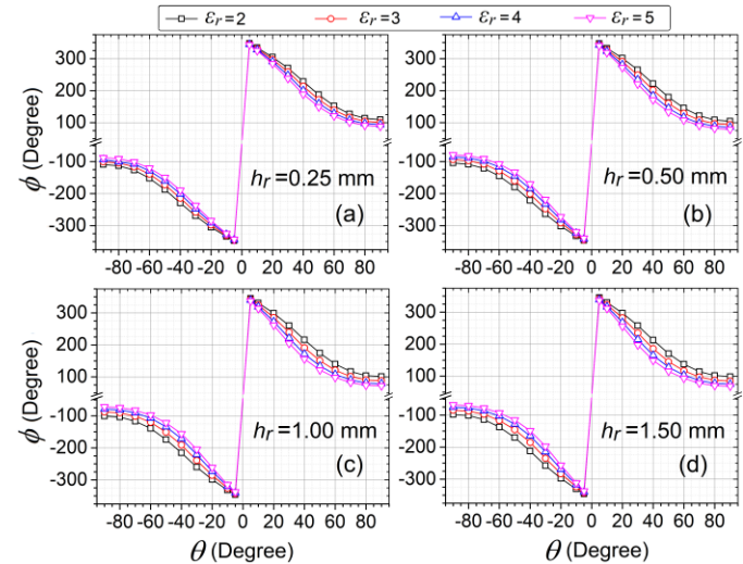
Figure 7. Relative phase of S_{11} and S_{22} calculated for various rotors with \epsilon_r = 2 to 5 and h_r = (a) 0.25 mm, (b) 0.50 mm (c) 1.0 mm, and (d) 1.50 mm, while \theta ranged from 0^\circ to \pm 90^\circ
