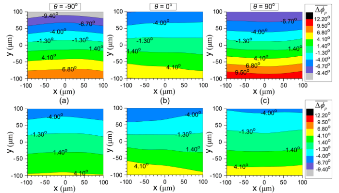
Figure 9. Positioning error for rotor1 with angular position (a) \theta = -90^\circ , (b) \theta = 0^\circ , (c) \theta = 90^\circ ; and for rotor2 with angular position (d) \theta = -90^\circ , (e) \theta = 0^\circ , and (f) \theta = 90^\circ .
