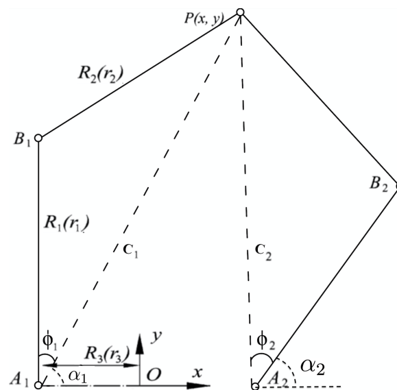
Figure 3. The planar 5R parallel mechanism.
