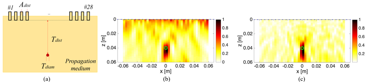
Figure 1. Simulation 1 . Sketch of the measurement scenario (a). Single-frequency reconstructions at 26.5 GHz. (b) Normalized LSM and (c) BA indicators. The target is superimposed as a green circle, while the antenna positions are depicted as blue points.
