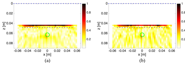
Figure 7. Measure3 . Normalized multifrequency BA indicators. (a) [18-40] GHz and N_F=276 , (b) [18-40] GHz and N_F=138 . The target is superimposed as a green circle, while the antenna and air-phantom interface positions are depicted as blue points.
