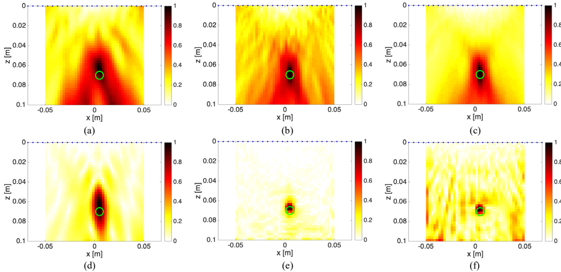
Figure 5. Measure1 . Normalized LSM (first row) and BA (second row) indicators. (a),(d) Single-frequency processing at 18 GHz. Multi-frequency processing involving a frequency range of [18-40] GHz: (b),(e) N_F=56 ; (c), (f) N_F=6 . The target is superimposed as a green circle, while the antenna positions are depicted as blue points.
