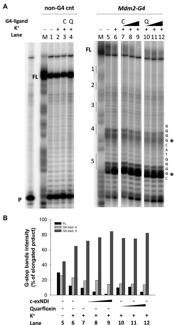
Figure 5. MDM2 G4 folds into multiple species. (A) Image of a typical Taq polymerase stop assay. Mdm2-G4 template was amplified by Taq polymerase at 56°C in the absence (lane 5) and presence (lane 6) of 20 mM K + , 12.5, 50 and 200 nM c-exNDI (lanes 7–9) and Quarfloxin (lanes 10–12). A template (non-G4 cnt) made of a scrambled sequence unable to fold into G4 was also used as negative control (lanes 1–4). Lane P: unreacted labeled primer. Lane M: ladder of markers obtained by the Maxam and Gilbert sequencing carried out on the amplified strand complementary to the template strand. Vertical bars indicate position of the G-tracts, while asterisks indicate G4-specific Taq polymerase stop sites. (B) Quantification of lanes 5–12 shown in panel A from two independent experiments. Quantification of stop bands corresponding to Mdm2-G4 and of the full-length amplification product (FL) is shown.
