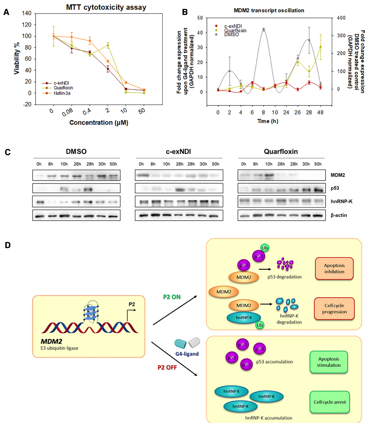
Figure 2. G4-ligands impair MDM2 transcription and restores the integrity of MDM2 target proteins in 93T449 cells. (A) MTT cytotoxicity assay upon 48 h treatment in the presence of c-exNDI, Quarflorin and Nutlin-3a. Compounds were tested in the 0.08–50 μM concentration range. (B) RT-PCR showing the fold change expression of MDM2 mRNA over time (0, 2, 4, 6, 8, 10, 24, 26, 28, 30, 50 h) upon treatment with the two G4-ligands c-exNDI and Quarflorin (55 nM) or DMSO treated control. Fold change expression values were internally normalized over GAPDH housekeeping mRNA and reported using the sample collected at 0 h from treatment as reference). The reported values represent the mean of three independent replicates with standard errors. Y-axis ranges are different for the G4-ligand treated samples (left axis) and DMSO control (right axis). (C) Western Blot analysis on cellular lysates to evaluate c-exNDI and Quarflorin (55 nM) effect over time (0, 8, 10, 12, 26, 28, 30, 50 h post-treatment) on MDM2 protein and its two targets p53 and hnRNP-K. DMSO treated lysate were evaluated as control sample. β-actin is shown as housekeeping gene. (D) Scheme of MDM2 pathways relative to its ubiquitin ligase activity on p53 and hnRNP-K, consequently inducing apoptotic arrest and stimulation of cell cycle progression (upper panel). Scheme of the proposed effect of G4-ligands on MDM2 P2-mediated transcription: the compound impairs Mdm2 transcription by binding to Mdm2 G4 (lower panel).
