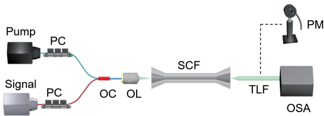
Fig. 4. The experimental setup for FWM in the tapered SCFs. PC, polarization controller; OC, optical coupler; OL, objective lens; TLF, tapered lens fiber; OSA, optical spectrum analyzer; PM, power meter.
