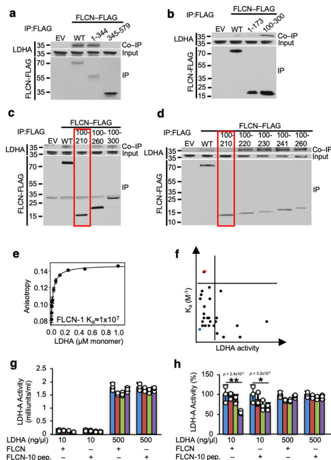
Extended Data Fig. 5 |. FLCN-10 peptide is able to effectively inhibit dimeric but not tetrameric LDHA.
