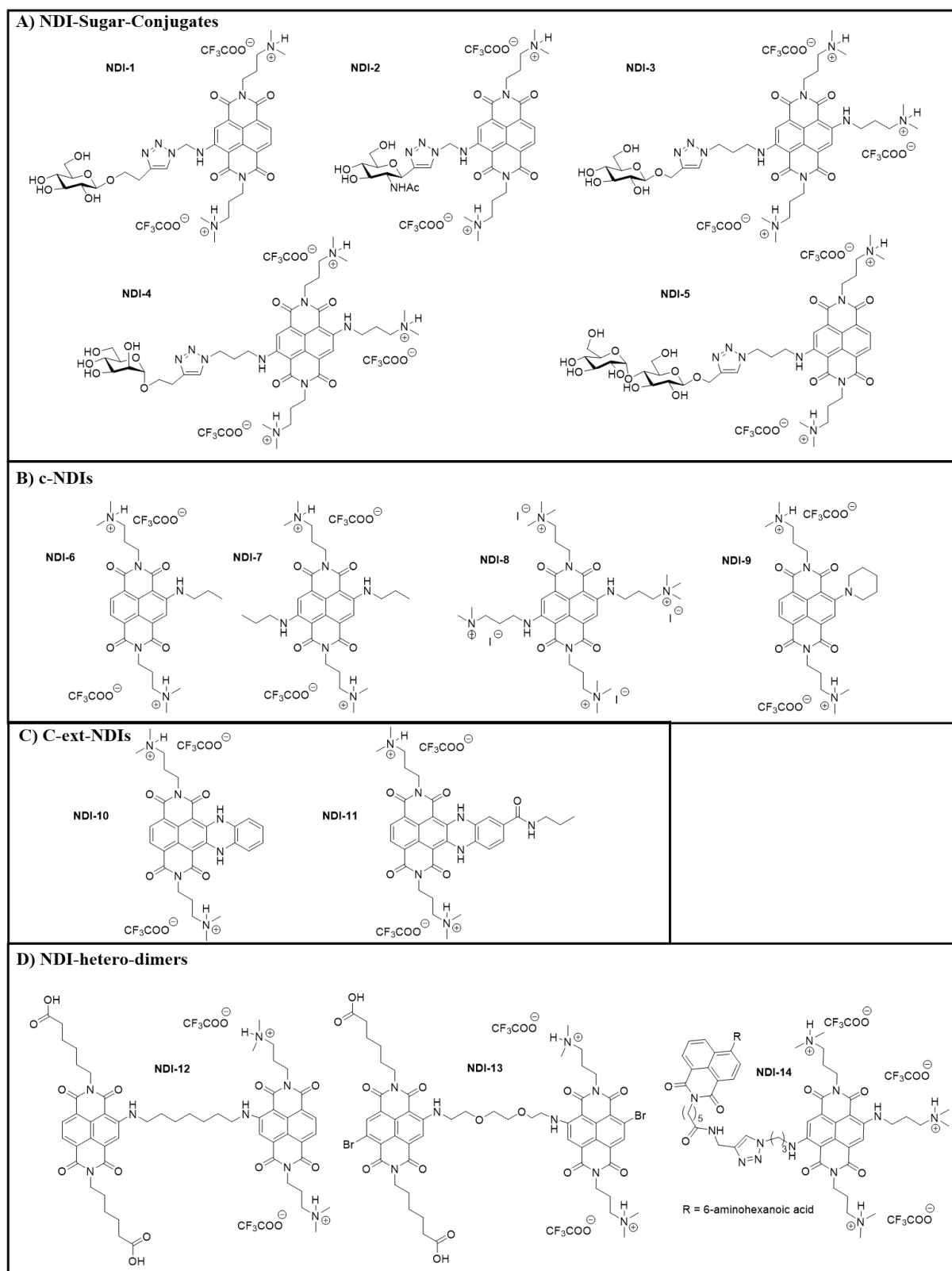
Figure 1. Chemical structures of A) NDI-Sugar conjugates ( NDI-1-5 ); B) core-substituted NDIs (c-NDIs; NDI-6-9 ); C) Core-extended NDI (C-ext-NDIs; NDI-10 and NDI-11 ); D) NDI-hetero-dimers ( NDI-12-14 ) synthesized and investigated in the present study.
