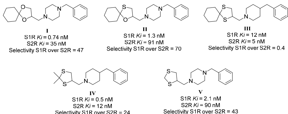
Fig. 2. S1R agonists currently in clinical trials: chemical structures, binding affinity at S1R and S2R and therapeutic indications.
