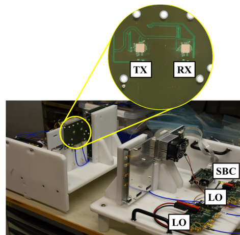
Fig. 22. Test bench for the D-band demo link trials.
