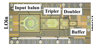
(e) Frequency sextupler. Size: 1.71 mm x 0.81 mm.
