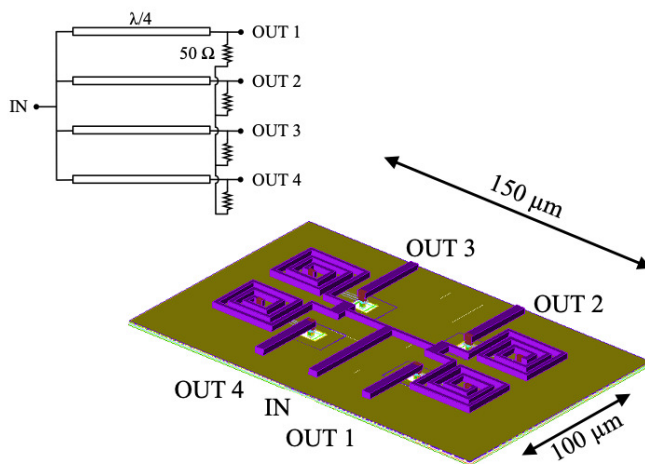
Fig. 3. 3D view of the implemented 4-way splitter.
