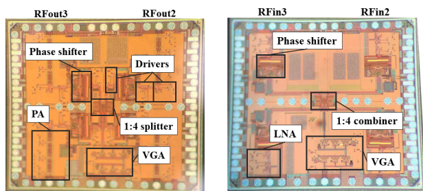
(a) 4-channel TX antenna driver. Size: 1.76 mm x 1.57 mm.
