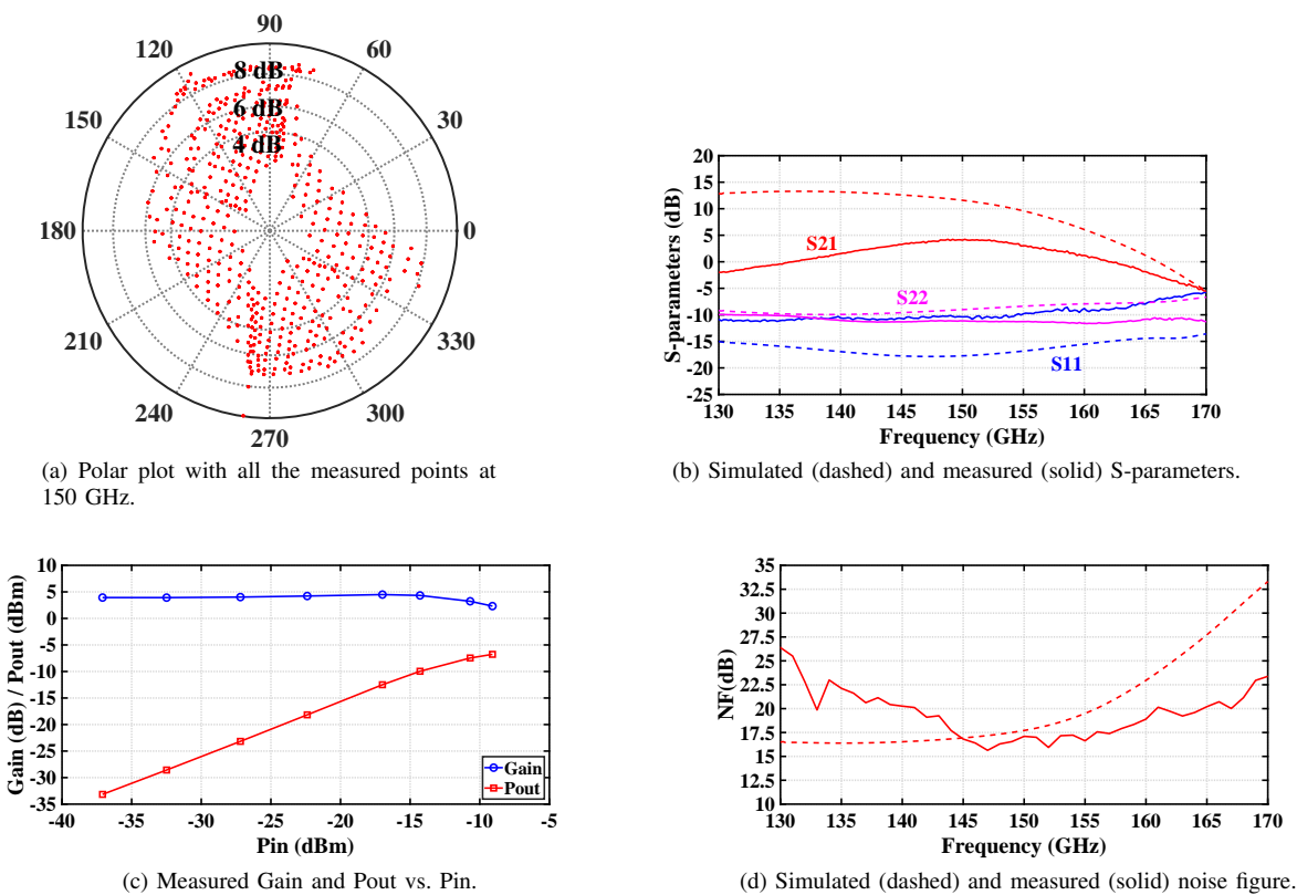
Fig. 16. Test results of a channel in the RX antenna driver chip.
