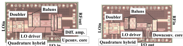
(c) I/Q up-converter. Size: 1.98 mm x 1.08 mm.
