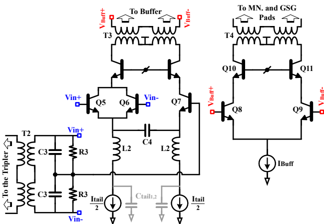
Fig. 12. Schematics of the proposed doubler and the output buffer of the sextupler.
