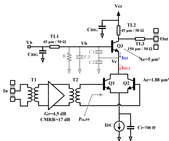
Fig. 13. Schematic of the proposed D-band frequency doubler.
