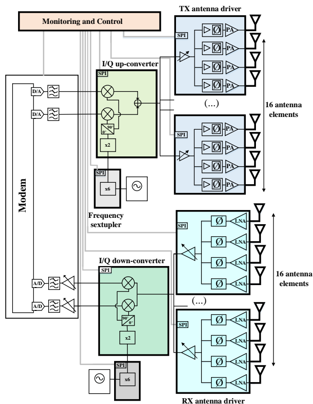
Fig. 2. Proposed transceiver architecture.
