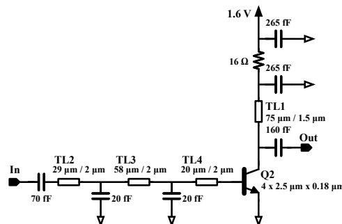
Fig. 5. Schematic of the last stage of the proposed PA.
