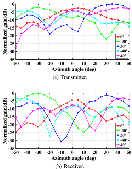
Fig. 23. Manually measured radiation patterns at 17 cm.
