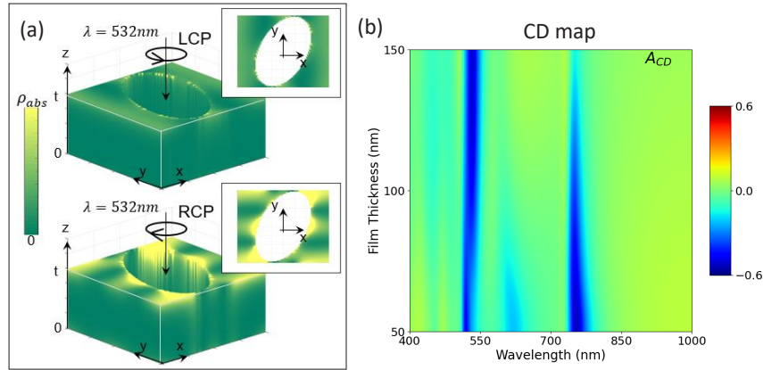
Fig. 8. Results for Ag: (a) 3D absorption density \rho_{abs} confinement in a unit cell, for LCP and RCP excitation at the wavelength of peak 1 for the optimized parameters in Fig. 7(a); 2D inset panels show the top surface view. (b) Absorption CD map as a function of Ag film thickness, keeping the same D_1, D_2, \phi as in Fig. 7(a).
