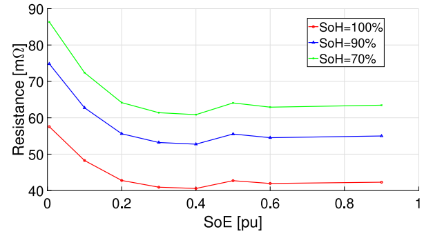
Fig. 4. Battery resistance value as function of SoE [58].
