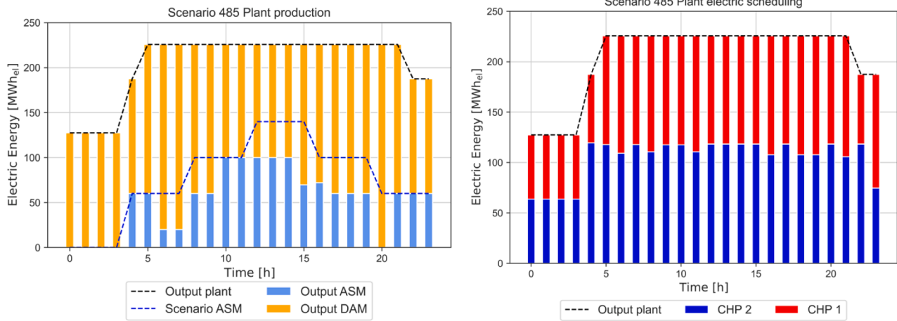
Fig. 21. Case 2 scenario 485, c_{NG} = 30\text{€/MWh} – Left: power plant electricity export; Right: power plant electricity scheduling.
