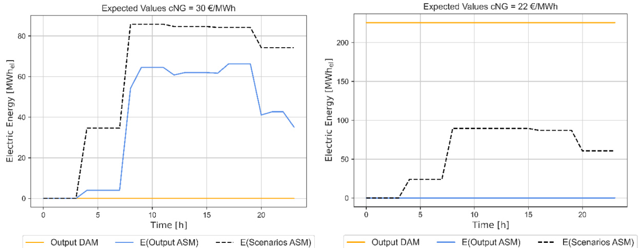
Fig. 18. Case 1 DAM and expected ASM bidding profiles. Left: c_{NG} = 30\text{€/MWh} ; Righth: c_{NG} = 22\text{€/MWh} .
