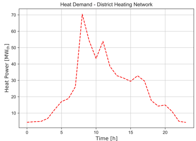
Fig. 16. Case 2 heat demand of the district heating network.
