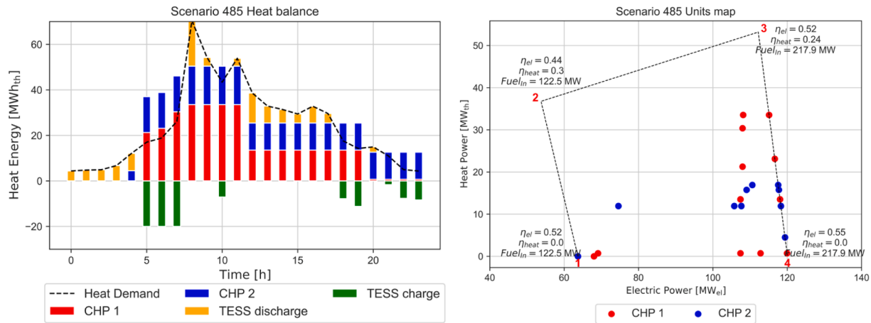
Fig. 22. Case 2 scenario 485, c_{NG} = 30€/MWh – Left: Heat balance; Right: CHPs operative points.
