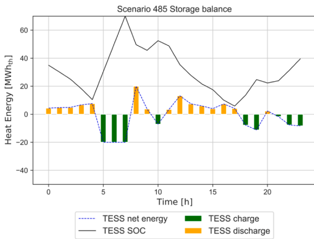
Fig. 23. Case 2 scenario 485, c_{NG} = 30€/MWh , storage operation.
