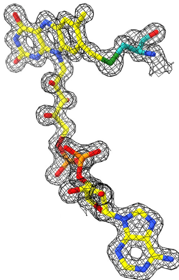
Fig. 8. Cys-FAD refined 2F o -F c electron density contoured at 1.5 σ. The FAD part is shown with carbon, oxygen, nitrogen, and phosphorus atoms in yellow, red, blue, and magenta, respectively. The covalently linked Cys394 is represented with carbon, oxygen, nitrogen, and sulfur atoms in light sea green, red, blue, and green, respectively. Structure was visualized using USCF ChimeraX [42].
