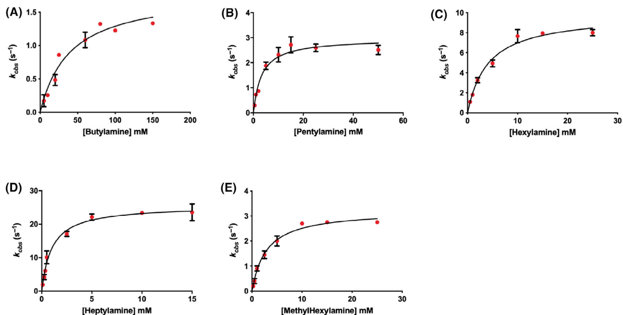
Fig. 5. Michaelis–Menten fitted curves of monoamine oxidase from Thermoanaerobacteriales bacterium (MAO Tb ) with the aliphatic monoamine substrates performed at the Oxygraph in 50 mM potassium phosphate buffer pH 7.5 (25 °C). All points for the different concentration of substrates were performed in duplicate. (A) n -butylamine. (B) n -pentylamine. (C) n -hexylamine. (D) n -heptylamine. (E) methyl hexylamine. Error bars indicate SD, and all points were taken in triplicates ( n = 3 ).
