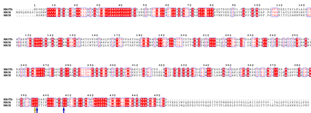
Fig. 1. Multiple sequence alignment of monoamine oxidase from Thermoanaerobacteriales bacterium (MAO Tb ), MAO A, and MAO B generated with ESript [24]. Conserved residues are shown with a red background. The conserved FAD-binding cysteine is marked with a yellow arrow and the aromatic cage with a blue arrow.
