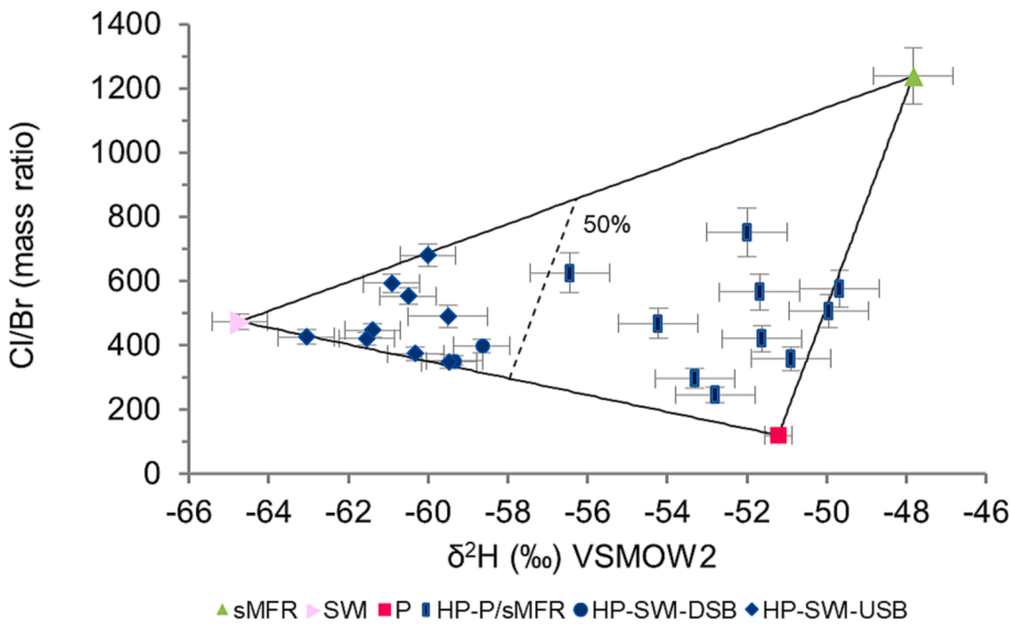
Fig. 2. Plot of Cl/Br vs \delta^2\text{H} for groundwater samples and mixing lines among end-members of recharge in the higher plain aquifer (see Sect. 3.2 for end-member composition). Error bars represent analytical errors. The percentage label on the mixing lines shows the fractional contribution to mixing of the end-member representing surface-water-irrigation. SWI: surface-water-irrigation. P: local precipitation. sMFR: surface mountain-front recharge. HP-P/sMFR: higher plain wells mainly recharged by local precipitation and/or surface mountain-front recharge; HP-SWI-USB: higher plain wells mainly recharged by surface-water-irrigation and located upstream of the springs belt; HP-SWI-DSB: higher plain wells mainly recharged by surface-water-irrigation and located downstream of the springs belt.
