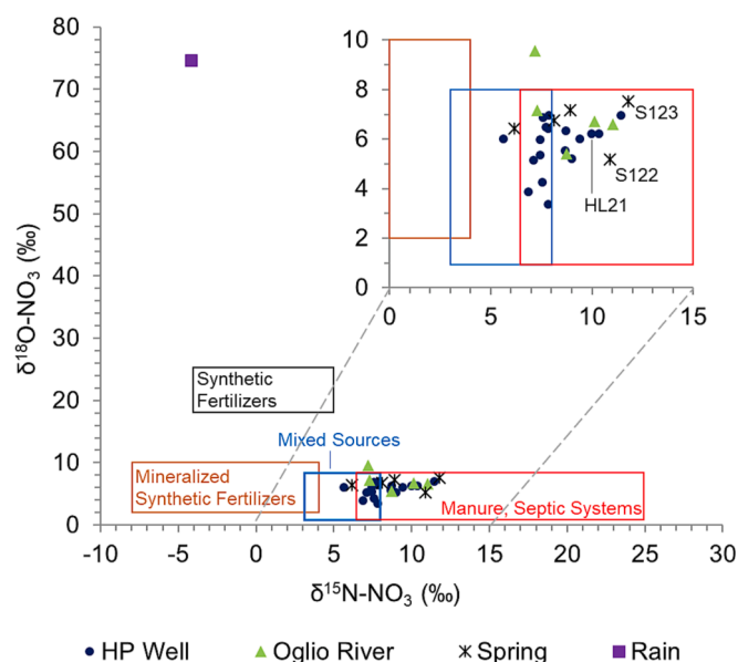
Fig. 6. Plot of \delta^{18}\text{O} vs \delta^{15}\text{N} in NO 3 for higher plain groundwater, Oglio River, spring and rain samples; compositional ranges are from Martinelli et al. (2018). Labels refer to point IDs mentioned in the text.
