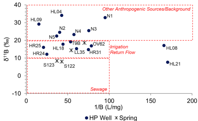
Fig. 7. Plot of \delta^{11}\text{B} vs 1/B for higher plain groundwater and spring samples; dotted red boxes represent the three groups described in Sect. 4.3. Labels refer to point IDs. (For interpretation of the references to color in this figure legend, the reader is referred to the web version of this article.)
