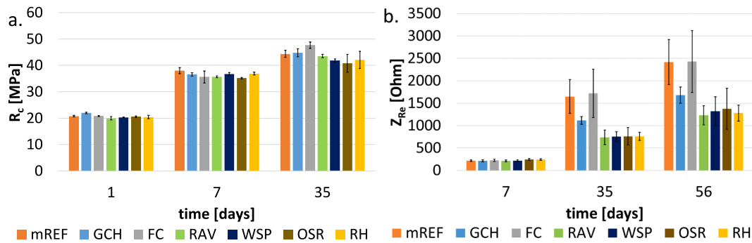
Fig. 6. a. compressive strength and b. electrical impedance of mortar specimens cast with different carbon-based fillers.
