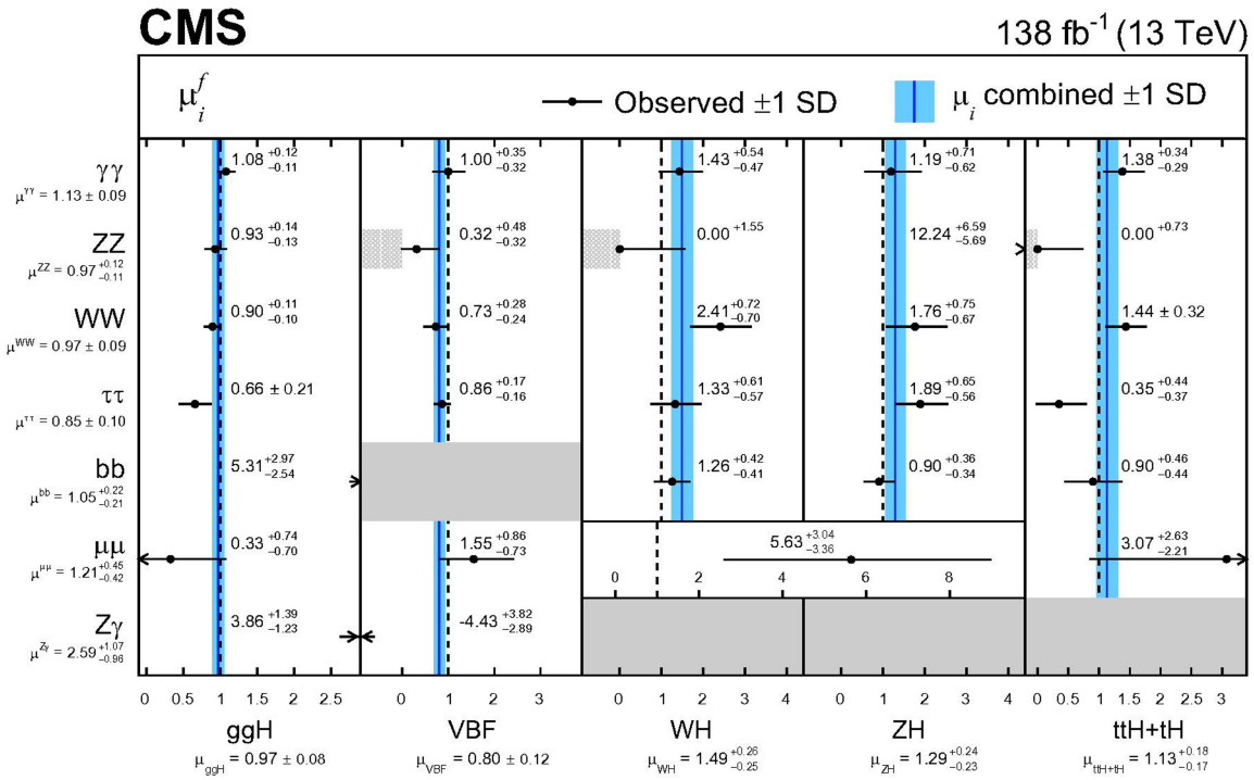
Extended Data Fig. 6 | The agreement with the SM predictions in Higgs boson production and decay. Signal-strength parameters per individual production mode and decay channel \mu_i^f , and combined per production mode \mu_i and decay channel \mu_i^f . In this fit, ttH and tH are considered together and the \mu_i
