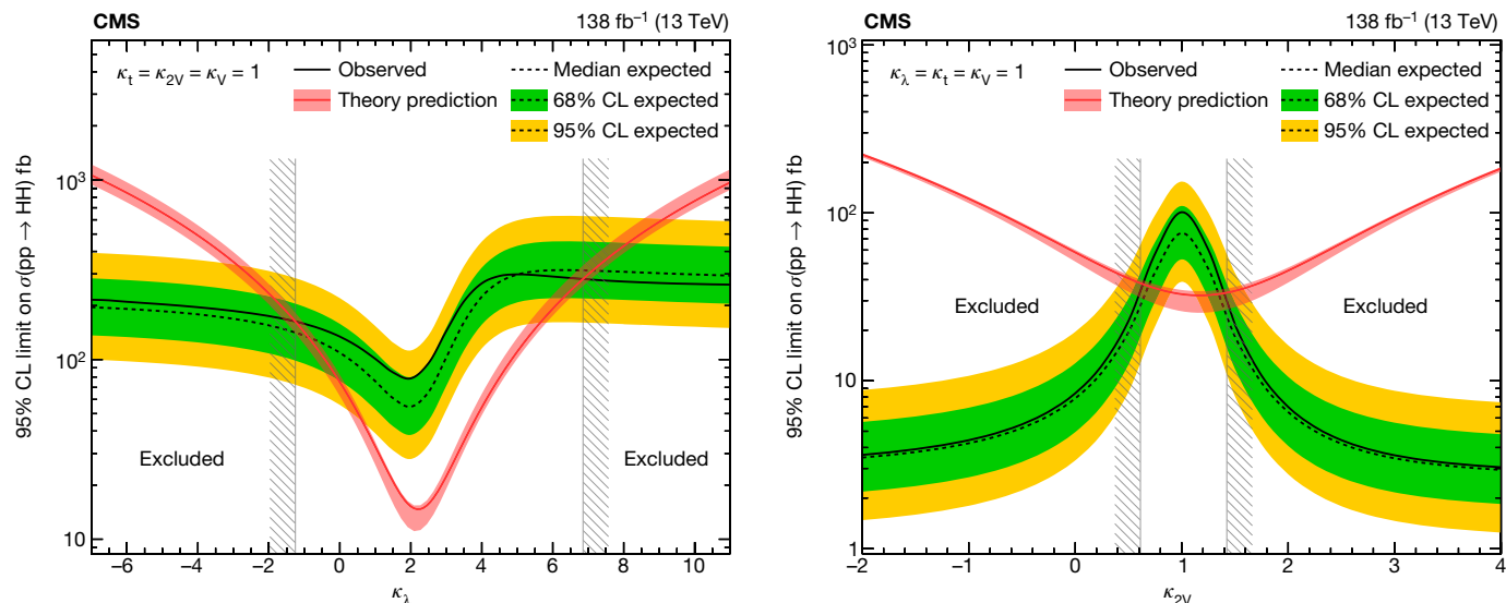
Fig. 6 | Limits on the Higgs boson self-interaction and quartic coupling. Combined expected and observed 95% CL upper limits on the HH production cross-section for different values of \kappa_\lambda (left) and \kappa_{2V} (right), assuming the SM values for the modifiers of Higgs boson couplings to top quarks and vector bosons. The green and yellow bands represent the 1-s.d. and 2-s.d. extensions
