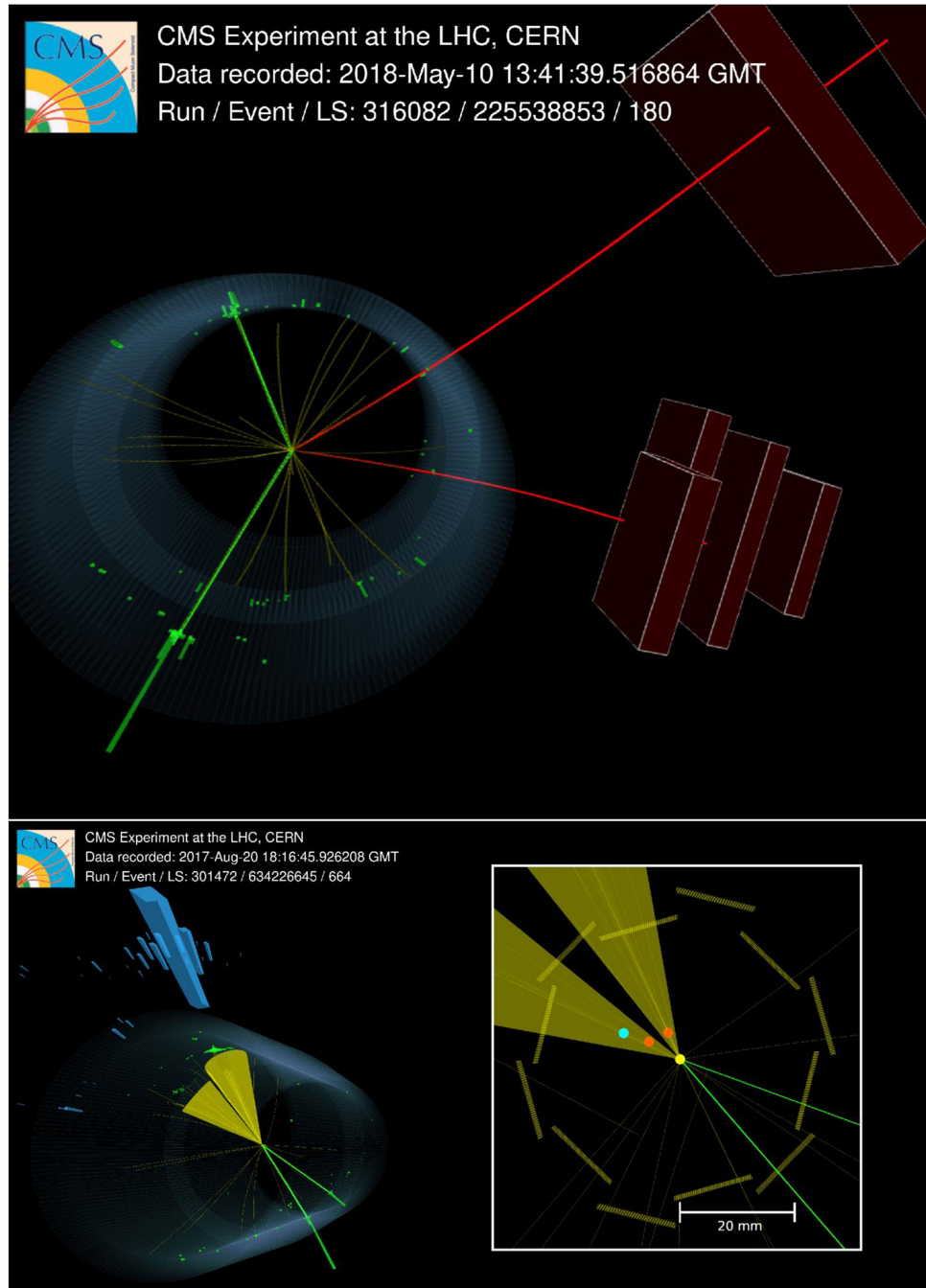
Extended Data Fig. 2 | Higgs boson candidate events. (upper) An event display of a candidate H \rightarrow ZZ \rightarrow e e \mu \mu . (lower) An event display of an H \rightarrow b b candidate produced in association with a boson decaying into an electron-positron pair, in pp collisions at \sqrt{s} = 13 TeV recorded by CMS. The charged-particle tracks, as reconstructed in the inner tracker, are shown in yellow; the electrons are shown in green, the energy deposited by the electrons in the ECAL is shown as large green towers, the size of which is proportional of the amount
