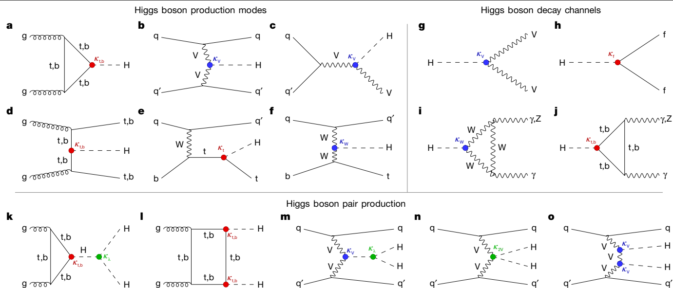
Fig. 1 | Feynman diagrams for the leading Higgs boson interactions. a–f , Higgs boson production in ggH ( a ) and VBF ( b ), associated production with a W or Z ( V ) boson ( VH ; c ), associated production with a top or bottom quark pair ( t\bar{t}H or b\bar{b}H ; d ) and associated production with a single top quark ( tH ; e , f ). g–j , Higgs boson decays into heavy vector boson pairs ( g ), fermion–antifermion pairs ( h ) and photon pairs or Z\gamma ( i , j ). k–o , Higgs boson pair production through
