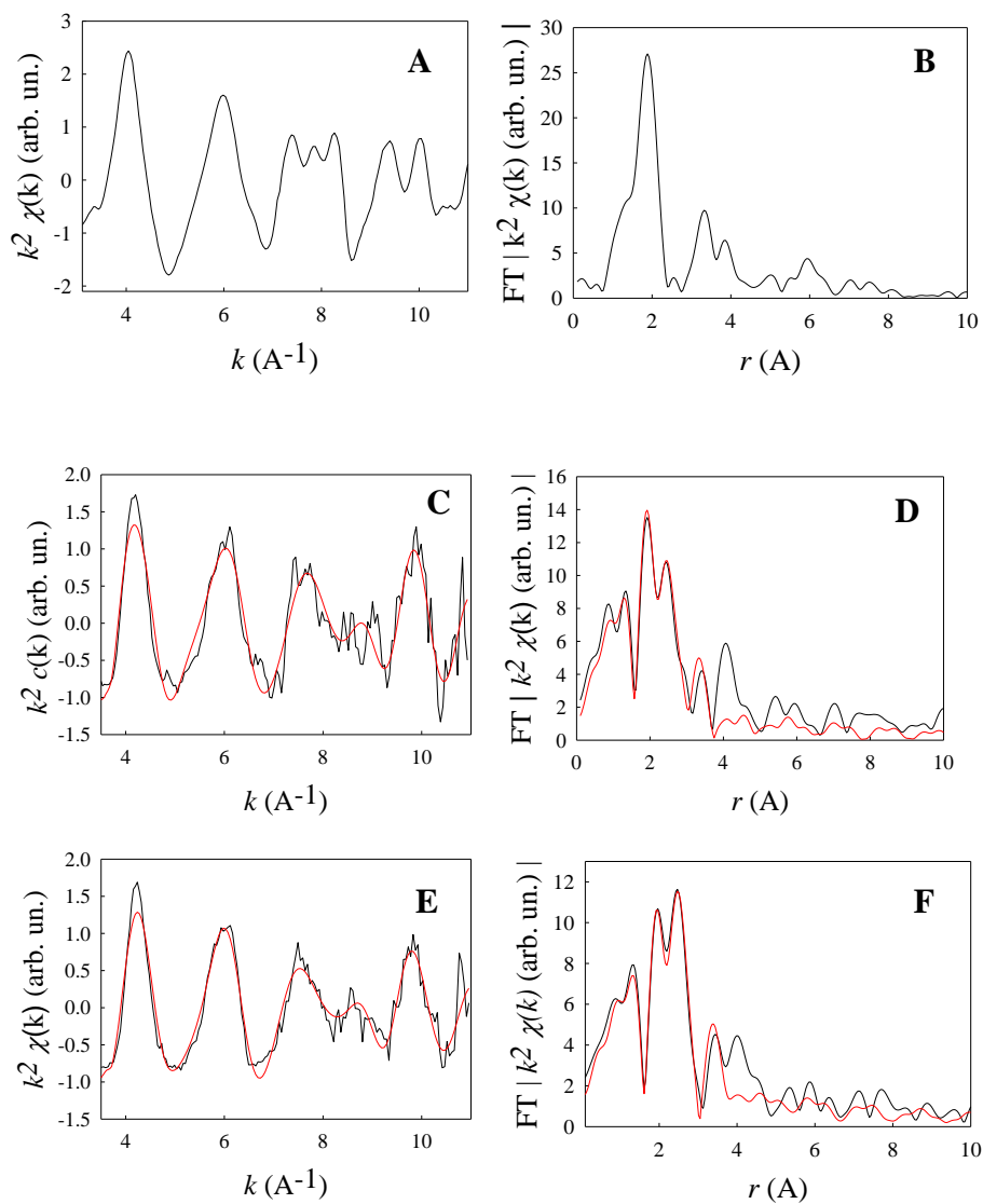
Figure 8: Ir-L III edge EXAFS signals and corresponding FT of IrO 2 (a and b) and of sample (e1_1) (c, d) and sample (e1_2) (e and f). The experimental signal is the black line while the fit according to the model described in the text is represented by the red line.
