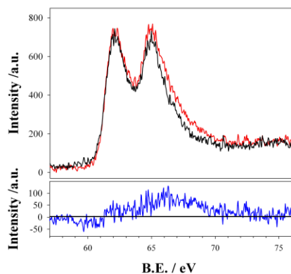
Figure 3: Normalized XPS spectra ( 4f_{7/2,5/2} ) of P1 (black line), P2 (red line) and their difference (blue line, bottom box) as a function of binding energy (BE). The intensity of difference was scaled by a factor 3 for better readability.
