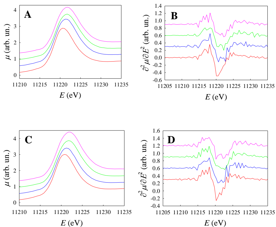
Figure 10: XANES spectra (A,C) and their second derivatives (B,D) of e1_1 (A,B) and e1_2 (C,D) after the subtraction of metallic iridium contribution. Spectra were acquired at 0.2 V (red line), 1.0 V (blue line), 1.3 V (green line) and 1.5 V (pink line).
