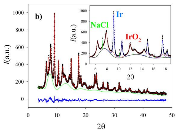
Figure 1. XRPD patterns of P1 (a) and P2 (b) samples. Experimental (black crosses) and calculated (red line) profiles are shown as well as background (green line) and residuals (blue line). The insets highlight the calculated contribution of the Ir (blue line), IrO 2 (red line) and NaCl (green line) phases.
