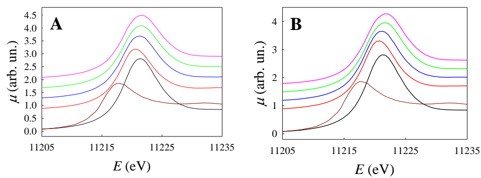
Figure 9: Ir L III edge XANES spectra of eI 1 (A) and eI 2 (B). Spectra were acquired at 0.2 V (red line), 1.0 V (blue line), 1.3 V (green line) and 1.5 V (pink line). The brown line is the spectrum of Metallic Ir and the black line is the spectrum of bulk IrO 2 , shown for reference.
