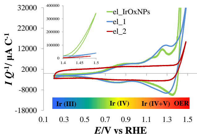
Figure 6: Cyclic voltammograms of el_1 (blue line), el_2 (red line) and el_IrO x NPs (green line) in aqueous 0.5 M H 2 SO 4 . Because of different loadings and for the sake of comparison (el_1 and el_2: 1 mg (Ir) cm -2 ; el_IrO x NPs: 0.01 mg (Ir) cm -2 ) currents have been normalized for the voltammetric charge. CVs are recorded at 2 mVs -1 . The inset displays the highest I window in the OER region. The color bar at the bottom aims to identify the Ir speciation prevalent in the potential window of interest, as highlighted in previous works. 11,24
