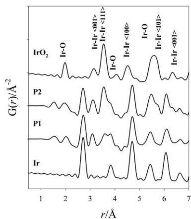
Figure 2. Experimental G(r) curves for P1 and P2 samples at short interatomic distances together with calculated G(r) for Ir and \text{IrO}_2 . For the \text{IrO}_2 phase, the couple of ions which contribute to each G(r) peak and the bond directions in respect to the crystalline axes are also reported.
