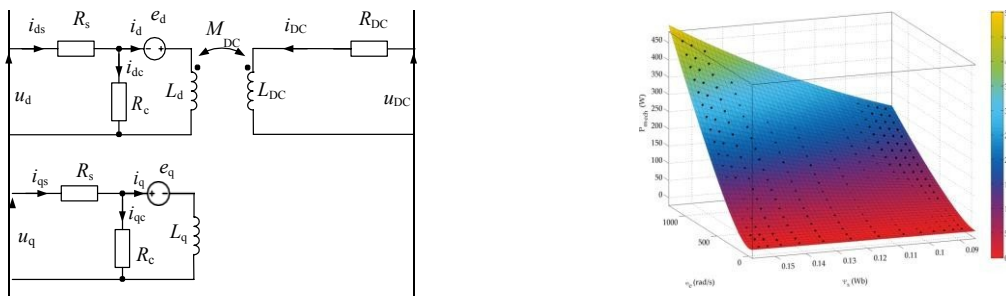
Fig. 5. Equivalent circuit of hybrid machine considering power losses in magnetic core (left). A result of match of mechanical and magnetic losses with measurement points (right).
