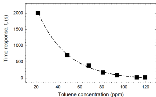
Figure 8: Time response of the nanocomposite sensor to different concentration of toluene vapor for a DBR having photonic band gap at 590 nm.
