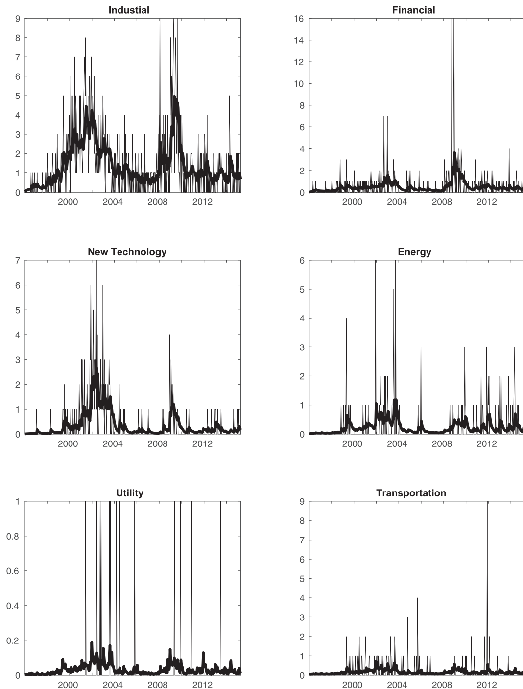
Fig. 5. Model 0 estimated intensities for the whole sample. This figure displays the implied \lambda s that are computed on the basis of the results displayed in Table 3 for the whole sample. The intensities (bold lines) are compared to the actual number of defaults (thin lines).
