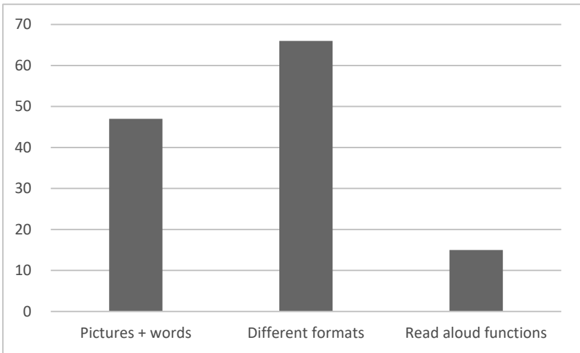
Figure 36 Multimodality
