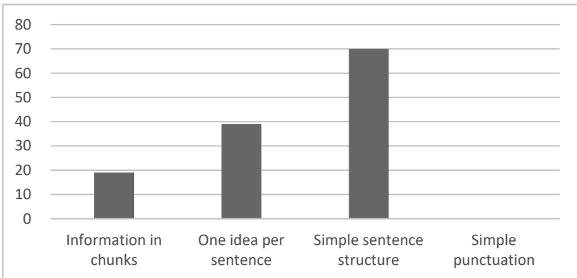
Figure 34 Syntax
