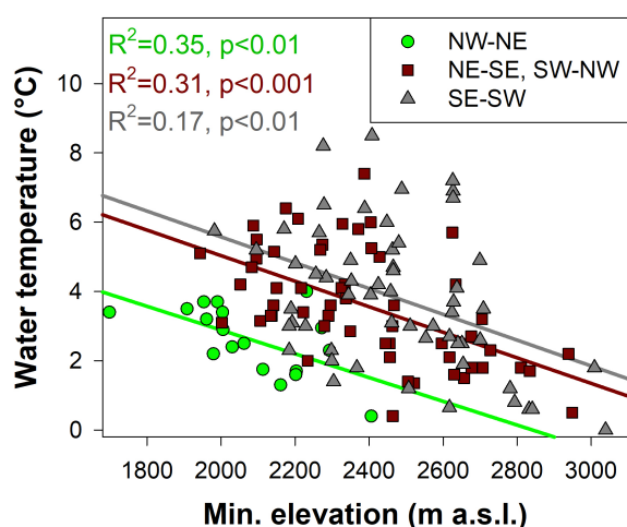
Figure 5. Relationship between spring-water temperature and minimum (spring) elevation, clustered into three classes of mean catchment aspect as in Fig. 4a.
