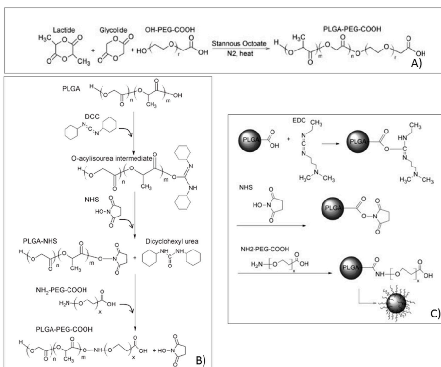
Figure 4. Poly(ethylene glycol) (PEG) conjugation to the poly(lactide-co-glycolide) (PLGA) polymer: (A) PEG conjugation throughout the PLGA polymerization reaction; (B) PEG conjugation to pre-made PLGA; (C) PEG conjugation to previously formed nanoparticles. (Modified from Bentacourt and co-workers. 2009 [57]).
