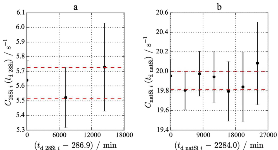
Figure 2. (a) ^{31}\text{Si} count rates of the ^{28}\text{Si} sample extrapolated at t_{d\ 28\text{Si}} = 286.9 min. (b) ^{31}\text{Si} count rates of the natSi sample extrapolated at t_{d\ \text{natSi}} = 2284.0 min. The error bars indicate a 95% confidence interval. The horizontal lines show the 95% confidence interval associated with the weighted mean of the count rate values.
