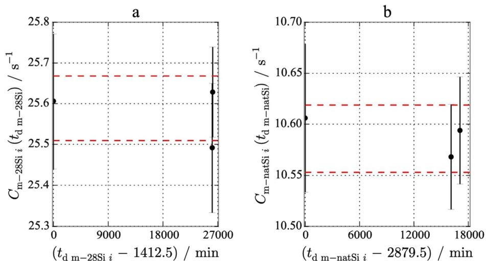
Figure 3. (a) ^{60}\text{Co} count rates of the monitor of the ^{28}\text{Si} sample extrapolated at t_{d\ m-28\text{Si}} = 1412.5 min. (b) ^{60}\text{Co} count rates of the monitor of the \text{natSi} sample extrapolated at t_{d\ m-\text{natSi}} = 2879.5 min. The error bars indicate a 95% confidence interval. The horizontal lines show the 95% confidence interval associated with the weighted mean of the count rate values.
