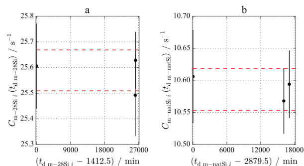
Figure 3. (a) ^{60}\text{Co} count rates of the monitor of the ^{28}\text{Si} sample extrapolated at t_{d\ \text{m-}28\text{Si}} = 1412.5 min. (b) ^{60}\text{Co} count rates of the monitor of the natSi sample extrapolated at t_{d\ \text{m-natSi}} = 2879.5 min. The error bars indicate a 95% confidence interval. The horizontal lines show the 95% confidence interval associated with the weighted mean of the count rate values.
